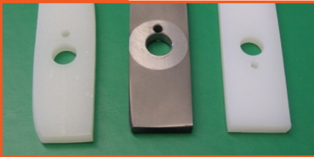
Test specimens of Sand-Slurry Test: GUR® UHMW-PE (on the right) shows the lowest abrasion values, compared to HDPE (left) and steel (middle).
