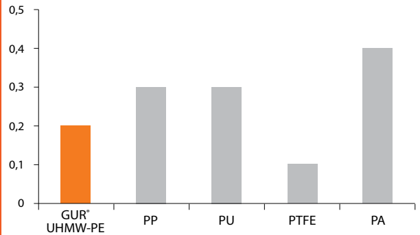
GUR® UHMW-PE is an excellent material for sliding applications, possessing self-lubricating properties, particularly in dry sliding movement against metal surfaces.
