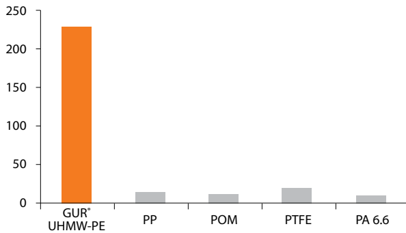
Results of modified „double notched“ Charpy impact test showing amount of energy absorbed by a material at the break point.
