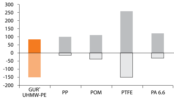
Typical operating temperature ranges for a selection of different materials.
