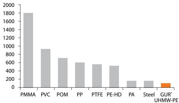
Material loss performance relative to GUR® UHMW-PE (=100) for different materials after a defined number of rotations in a sand-water mixture.
