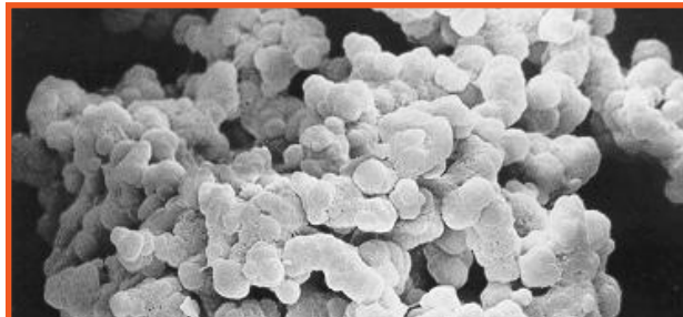
GUR® 2122 powder with a bulk density of >230 g/l prior to molding
