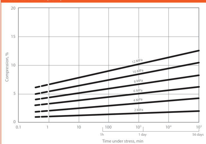
Figure 6 • Creep properties of UHMWPE under varying compressive stress rates, measured at 20 °C (68 °F)
