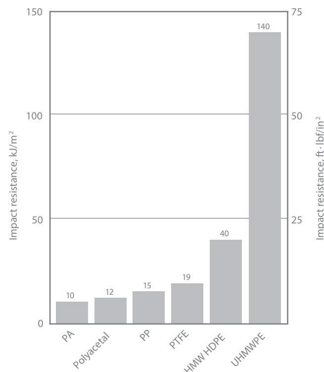
Figure 2 • Comparative impact resistance of different engineering resins
