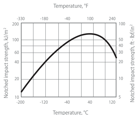
Figure 3 • Notched impact strength of UHMWPE as a function of temperature, using sharp V-notched test bar with double 15°V-notch
