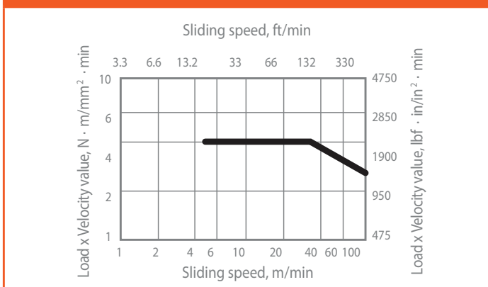
Figure 5 • Load limits for unlubricated bearings made from UHMWPE
