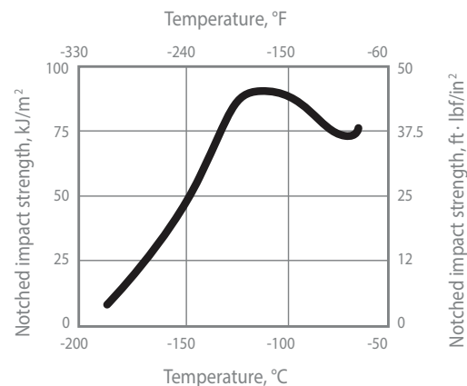
Figure 4 • Notched impact strength of UHMWPE as a function of temperature, based on a single 45°V-notch
